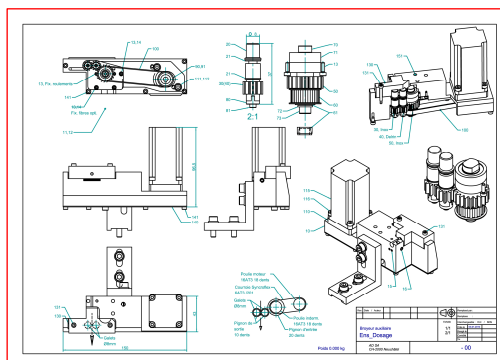
Mechanical plans - Subset plans -
