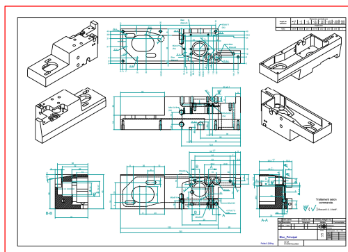
Mechanical plans - Detail machining -
